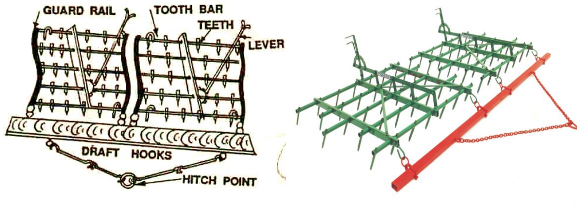
Fig. 14.5 line diagram of Spike tooth harrow
