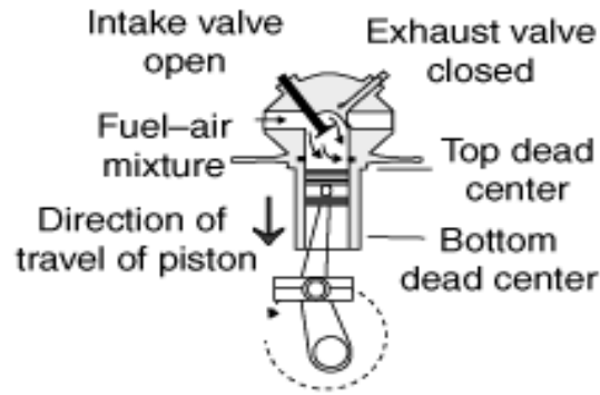
Induction stroke.
