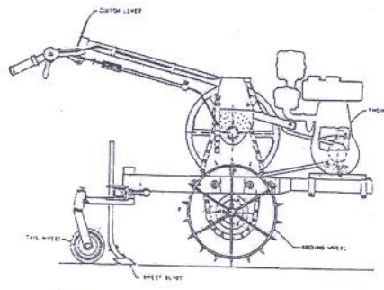
Fig. 18.2 Engine operated weeder
