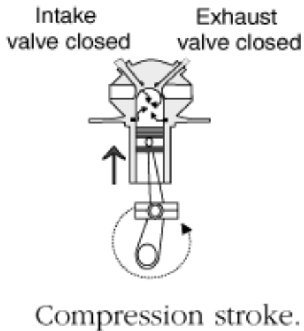
Fig. 3.2. Compression stroke
