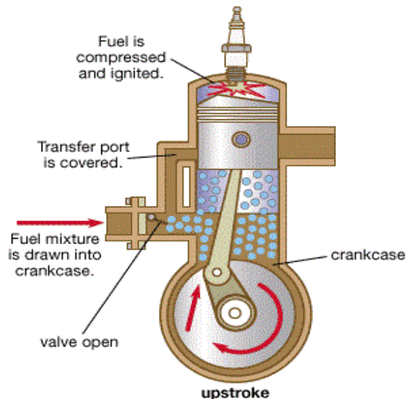
Plate : 3.2 First stroke in two stroke engine
