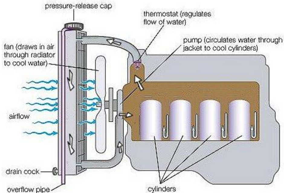
Fig. 5.4 Pressurized cooling system
