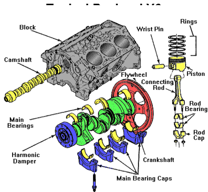
Plate : 2.15 Different parts of the engine
