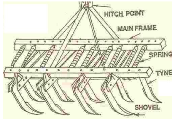
Fig. 15.1 Tractor drawn cultivator
