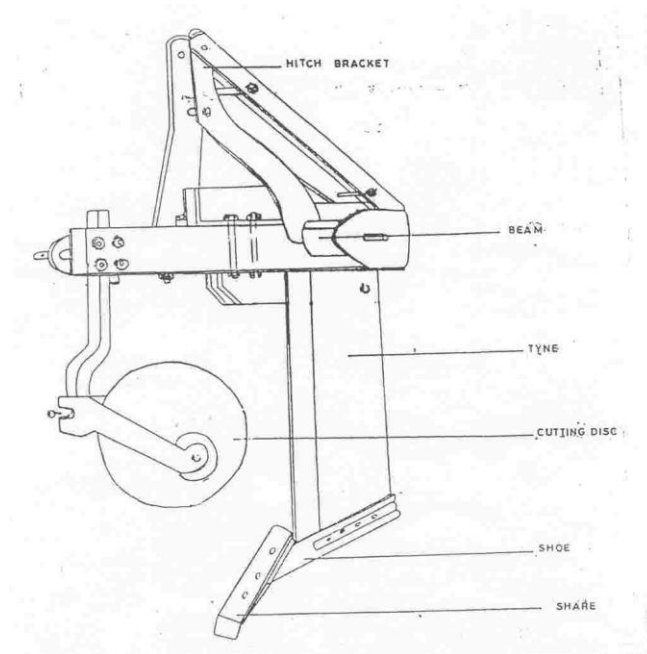
Fig. 13.4 Line diagram of Sub soiler
