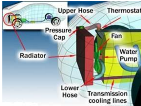
Fig. 5.3 Forced circulation system
