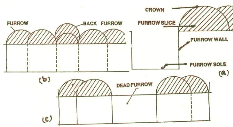
Fig. 11.1 Line diagram of different terminology used in ploughing
