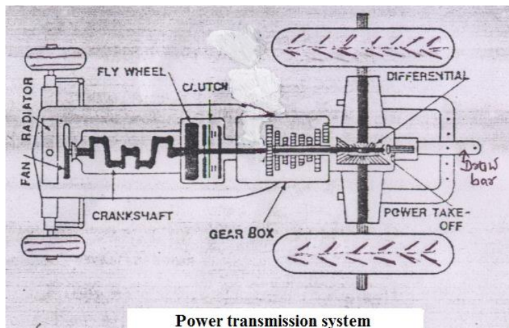
Fig. 7.1 Power transmission system
