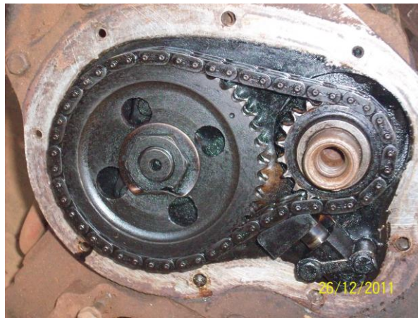
Plate : 2.13 A view of timing gear and chain arrangement
