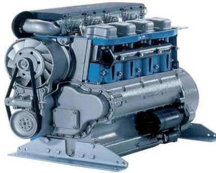
Plate : 2.2 Multi cylinder engine
