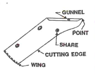
Fig. 12.2 Different parts of the share
