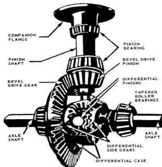
Fig. 7.2 Differential unit
