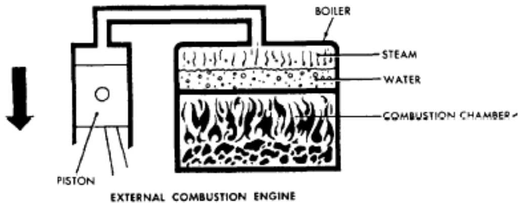
Fig 2.1. Working principle of External combustion engine.
