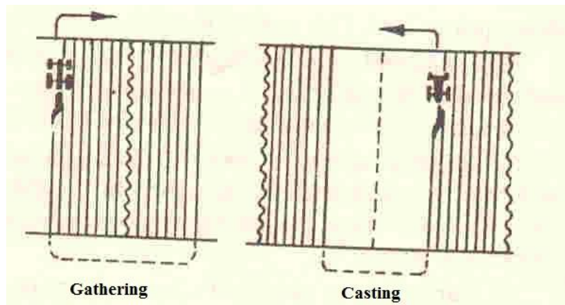
Fig.9.2 Line diagram of ploughing methods
