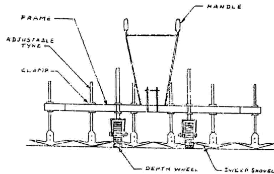
Fig. 18.3 Bullock operated sweeps
