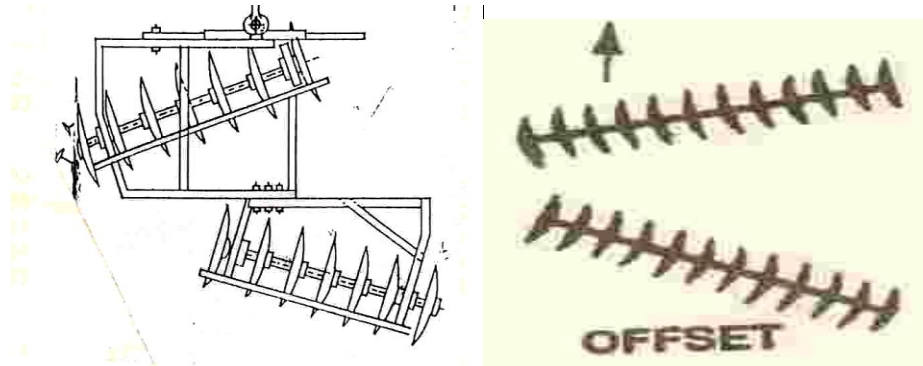
Fig. 14.4 line diagram of disc arrangement in offset disc harrow
