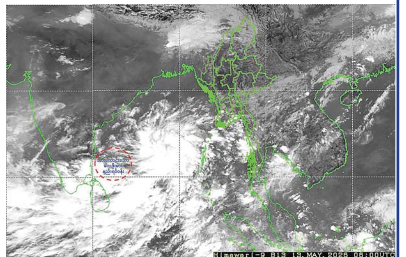
Himawari-9 B13 13 MAY 2025 06:00UTC
